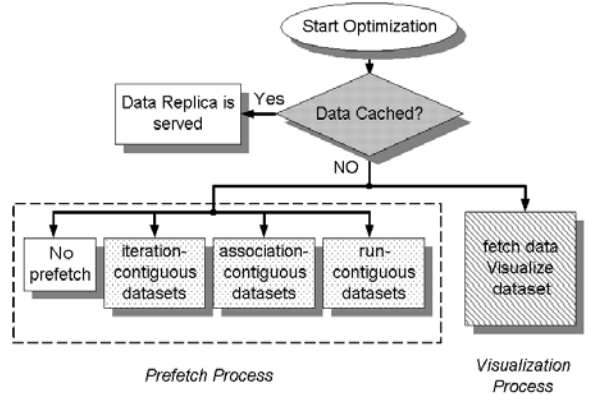
Figure 3. Optimizations in IJ-GUI.
