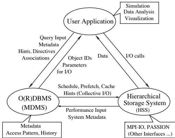
Figure 1. Three-tiered architecture.
